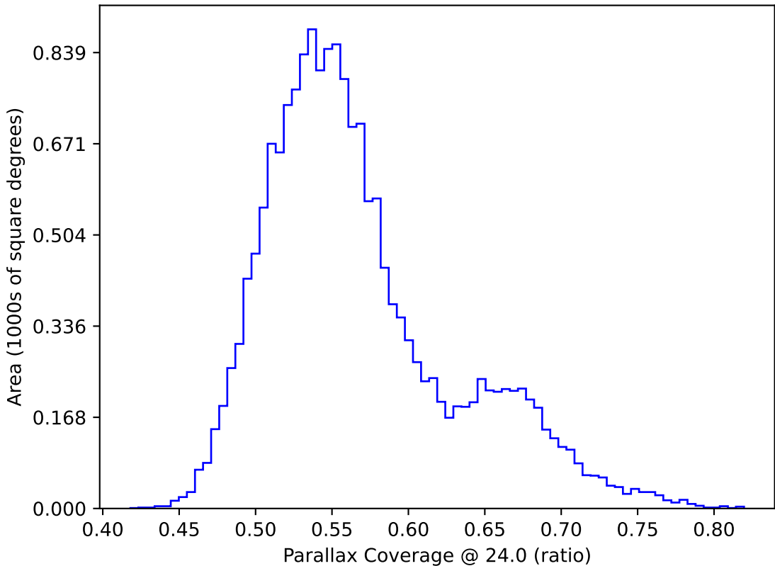
roll_pause_mjdp0_v3.4_10yrs WFD: Parallax Coverage @ 24.0
