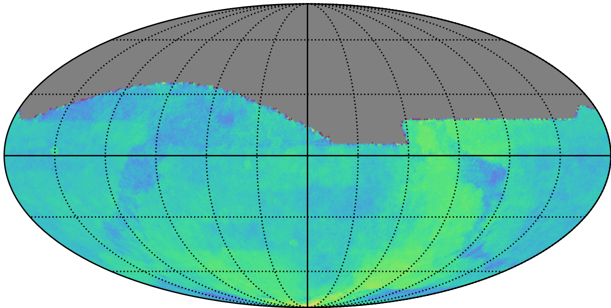
roll_pause_mjdp0_v3.4_10yrs All sky: Parallax Coverage @ 24.0
