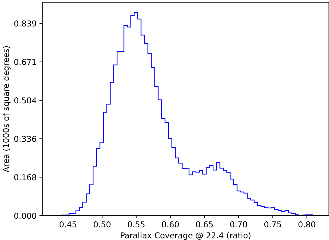
roll_pause_mjdp0_v3.4_10yrs WFD: Parallax Coverage @ 22.4
