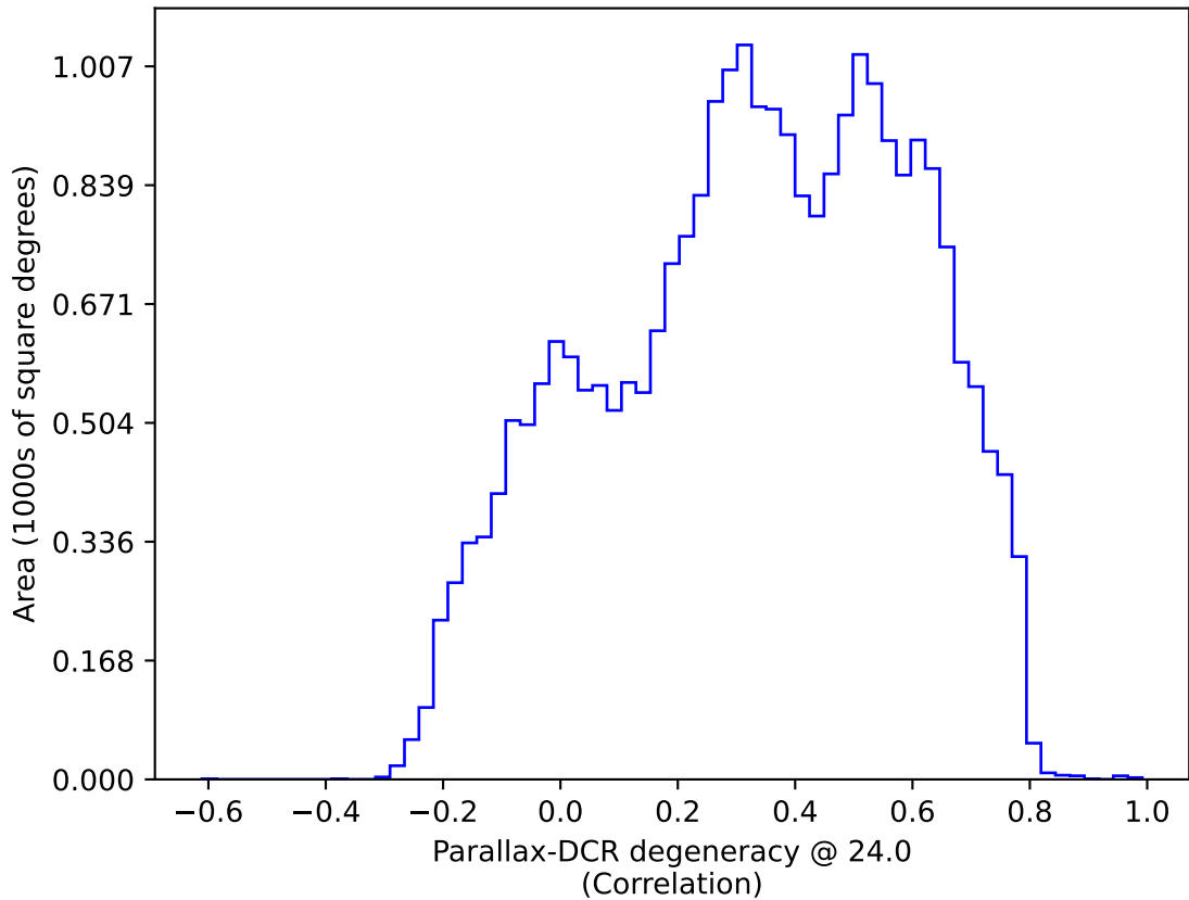
roll_pause_mjdp0_v3.4_10yrs All sky: Parallax-DCR degeneracy @ 24.0
