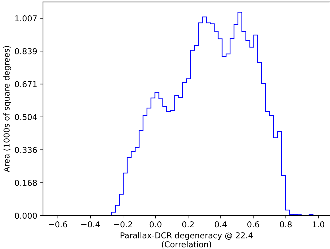
roll_pause_mjdp0_v3.4_10yrs All sky: Parallax-DCR degeneracy @ 22.4
