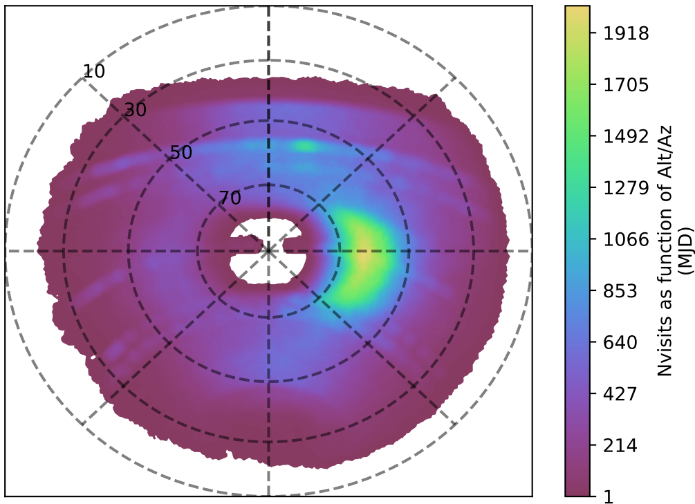
roll_pause_mjdp0_v3.4_10yrs y band: Nvisits as function of Alt/Az
