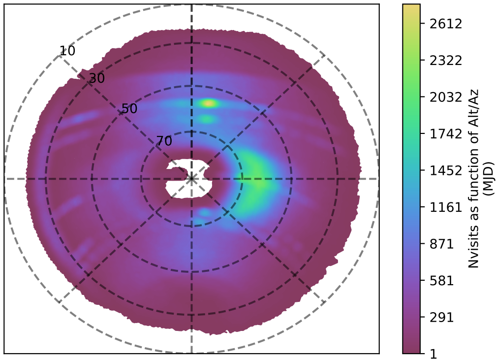
roll_pause_mjdp0_v3.4_10yrs r band: Nvisits as function of Alt/Az
