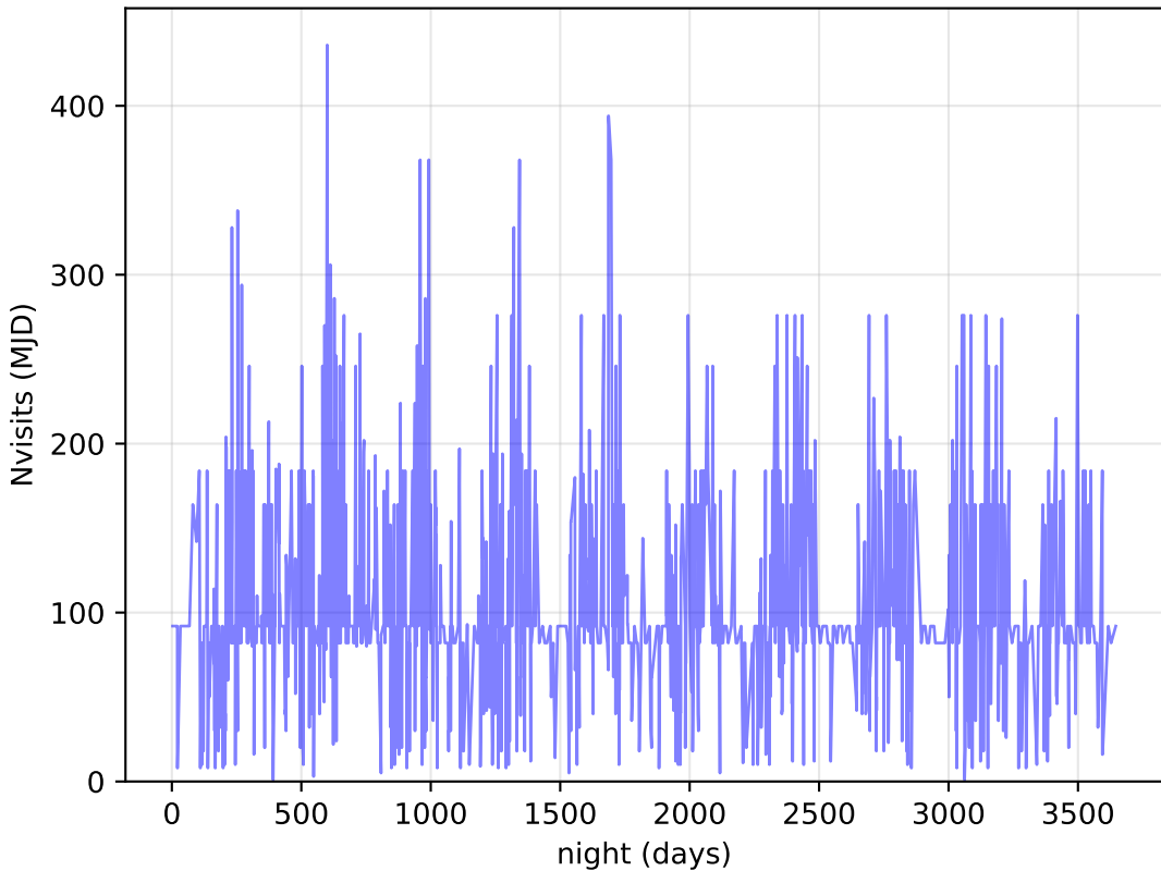
roll_pause_mjdp0_v3.4_10yrs DDF: Nvisits
