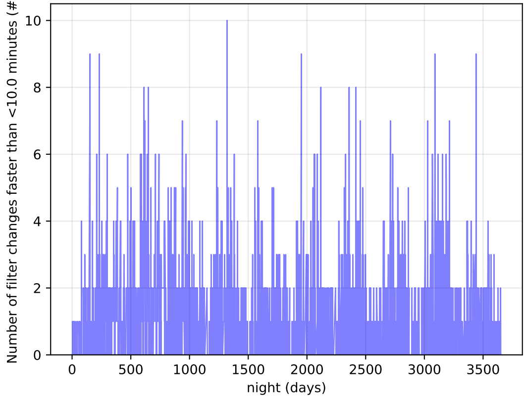
roll_pause_mjdp0_v3.4_10yrs Per Night: Number of filter changes faster than <10.0 minutes
