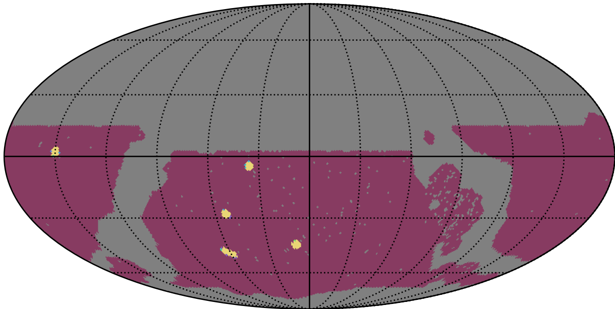
roll_pause_mjdp0_v3.4_10yrs WFD: NumberOfQuickRevisits
