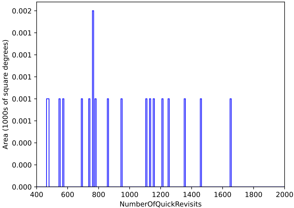
roll_pause_mjdp0_v3.4_10yrs WFD: NumberOfQuickRevisits
