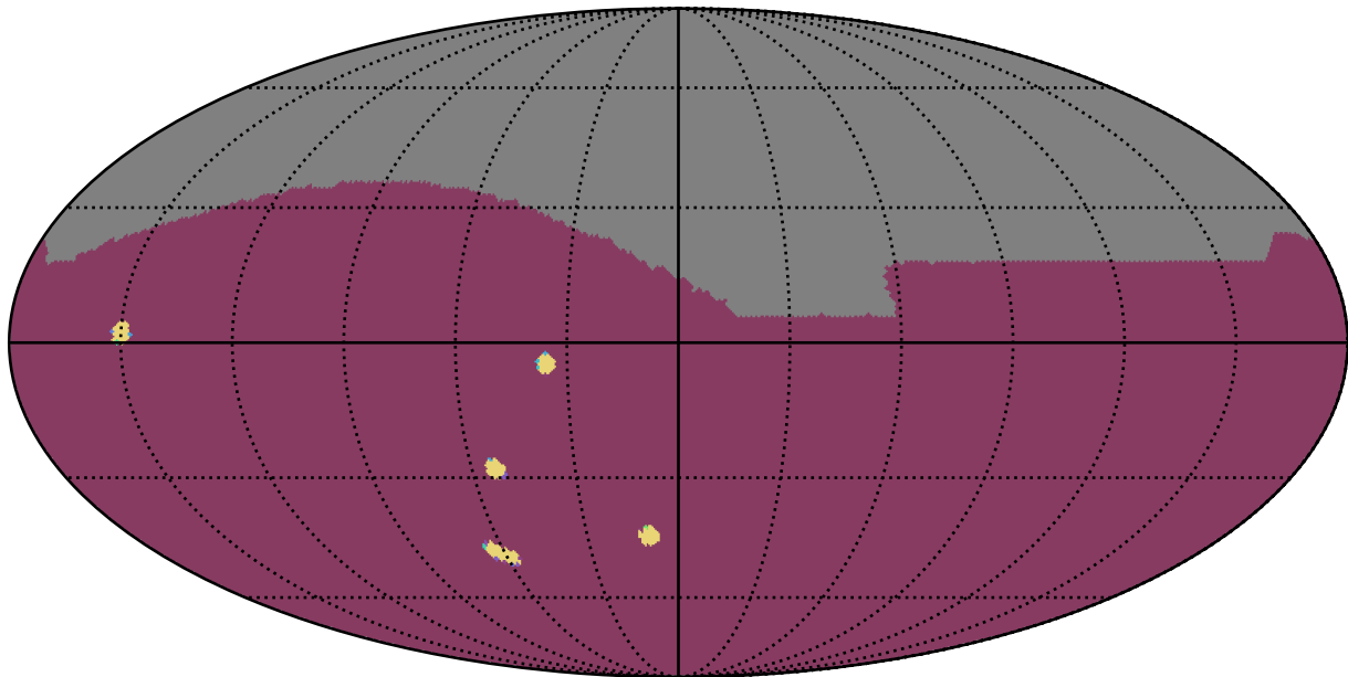
roll_pause_mjdp0_v3.4_10yrs All sky: NumberOfQuickRevisits
