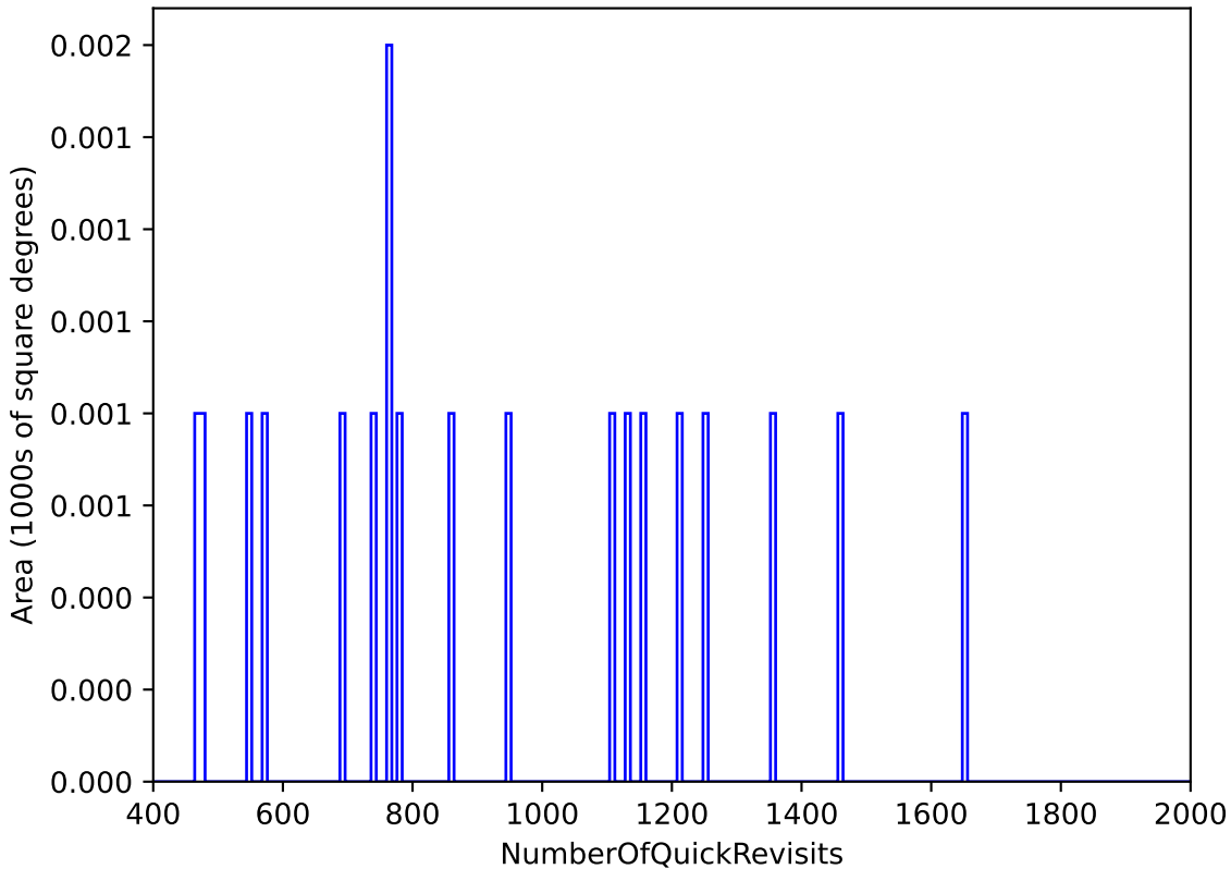
roll_pause_mjdp0_v3.4_10yrs All sky: NumberOfQuickRevisits
