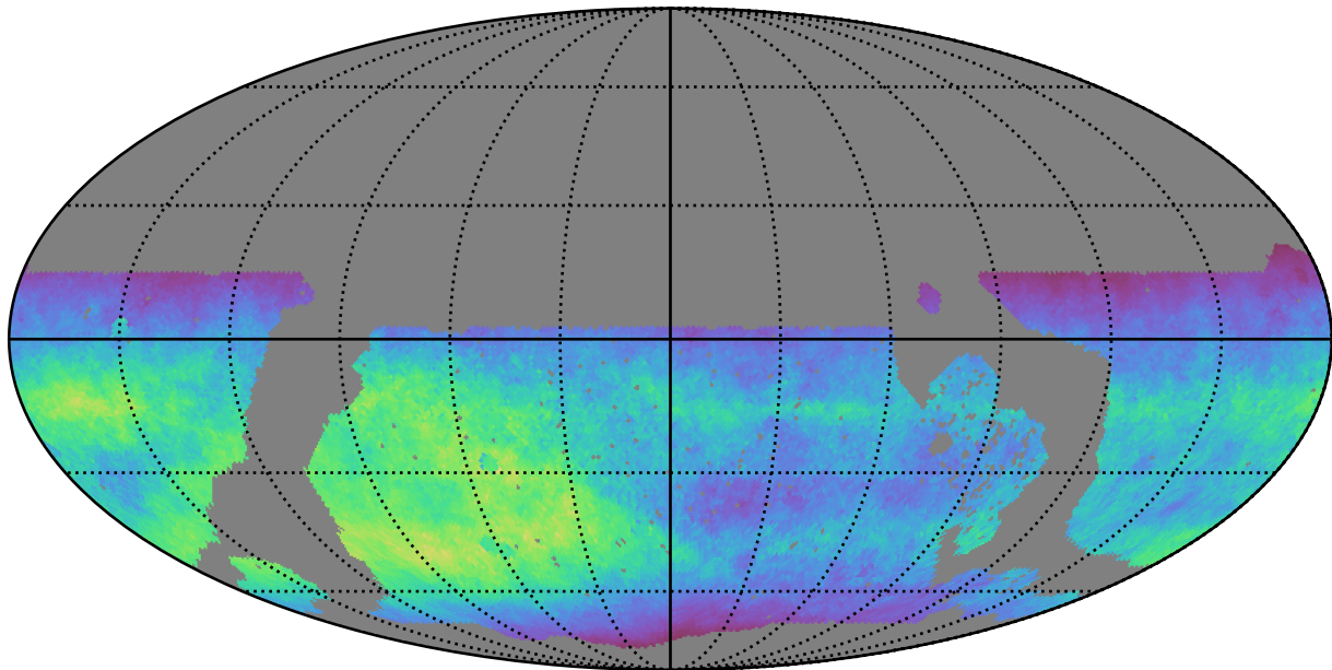
roll_pause_mjdp0_v3.4_10yrs WFD z band: Normalized Teff
