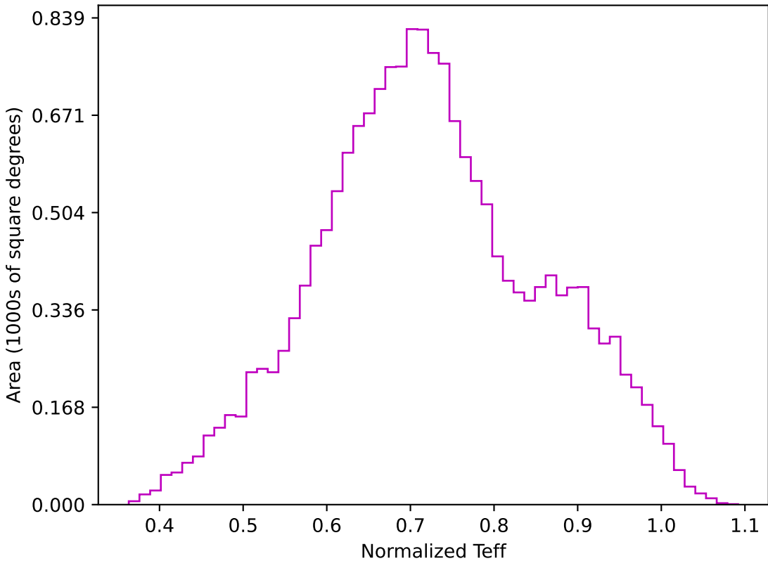
roll_pause_mjdp0_v3.4_10yrs WFD z band: Normalized Teff
