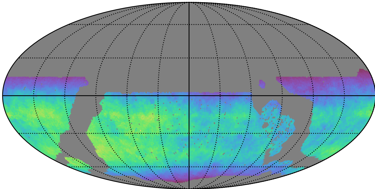
roll_pause_mjdp0_v3.4_10yrs WFD y band: Normalized Teff
