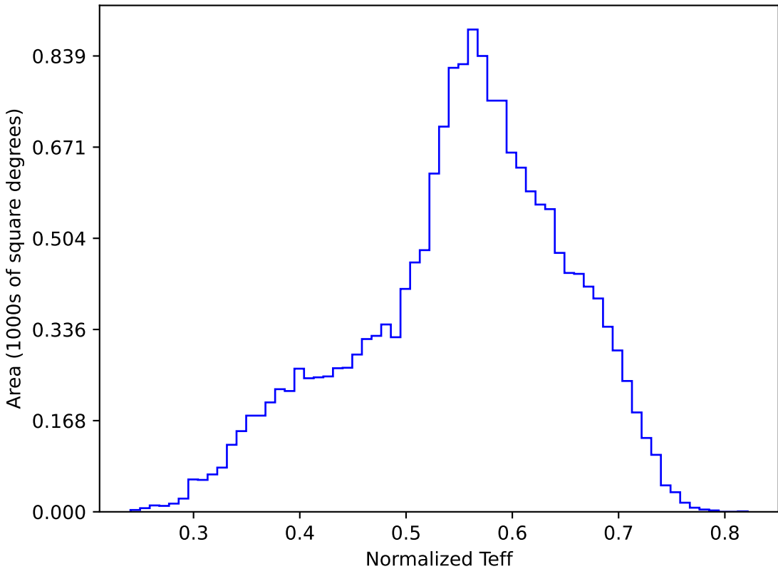
roll_pause_mjdp0_v3.4_10yrs WFD y band: Normalized Teff
