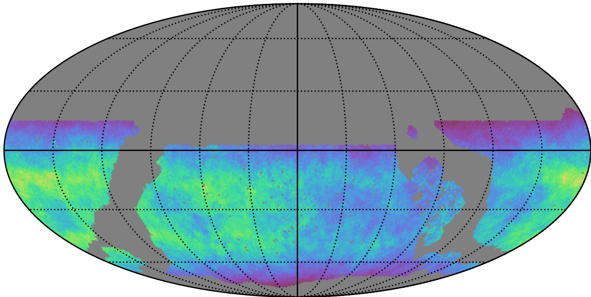
roll_pause_mjdp0_v3.4_10yrs WFD u band: Normalized Teff
