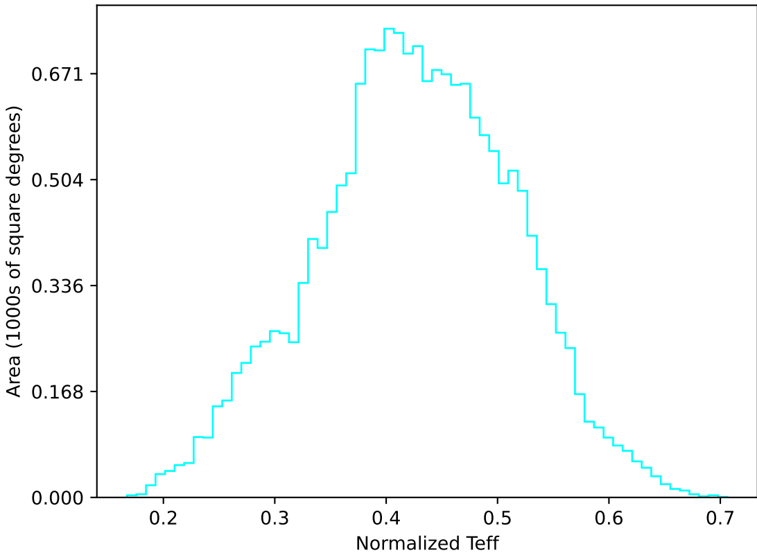
roll_pause_mjdp0_v3.4_10yrs WFD u band: Normalized Teff
