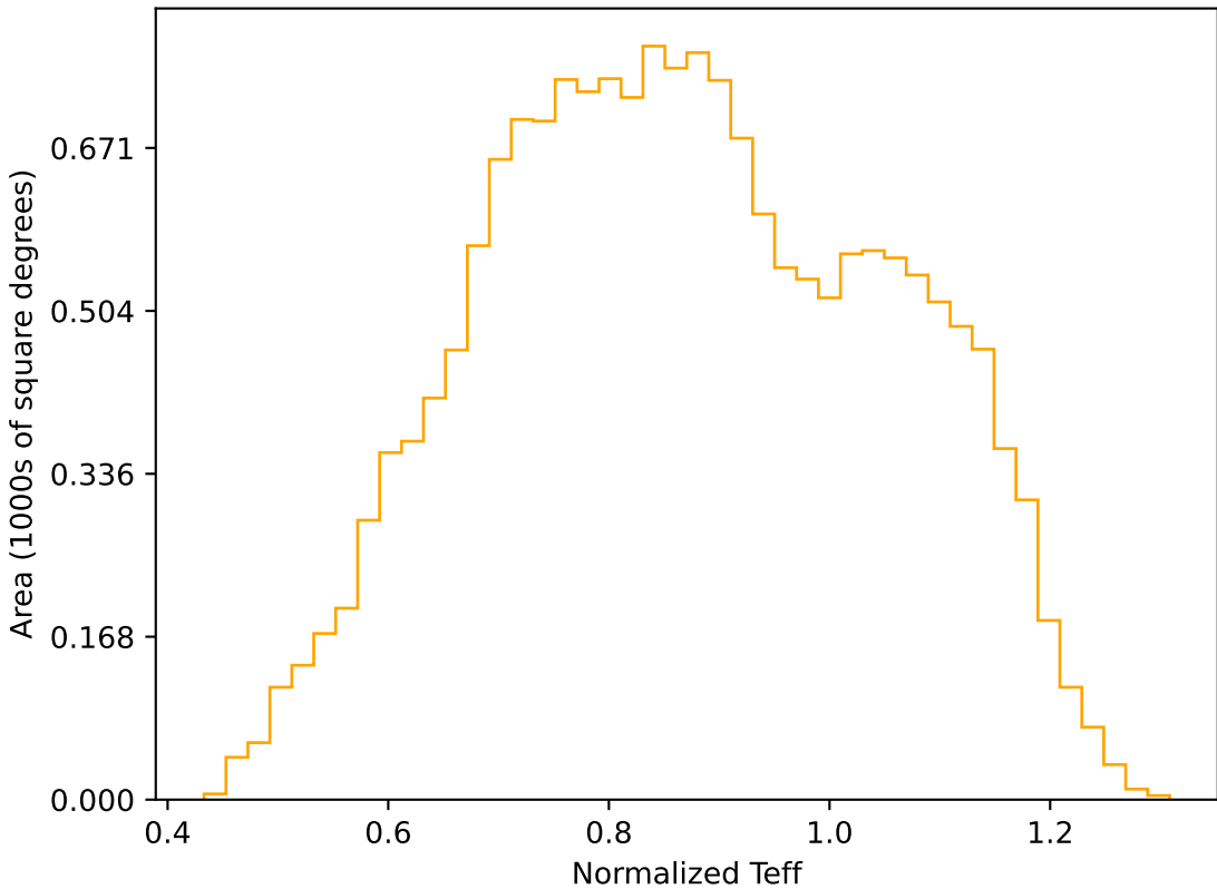
roll_pause_mjdp0_v3.4_10yrs WFD r band: Normalized Teff
