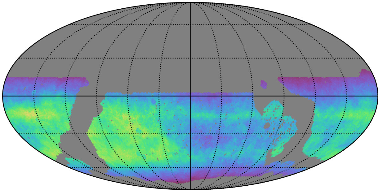
roll_pause_mjdp0_v3.4_10yrs WFD i band: Normalized Teff
