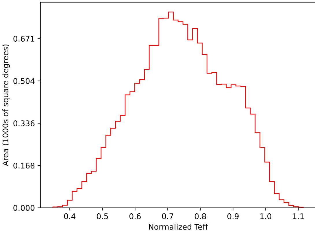
roll_pause_mjdp0_v3.4_10yrs WFD i band: Normalized Teff
