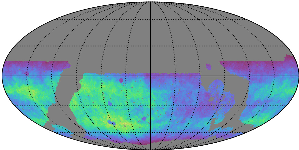
roll_pause_mjdp0_v3.4_10yrs WFD g band: Normalized Teff
