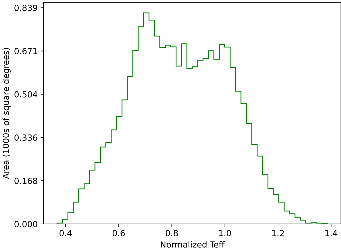
roll_pause_mjdp0_v3.4_10yrs WFD g band: Normalized Teff
