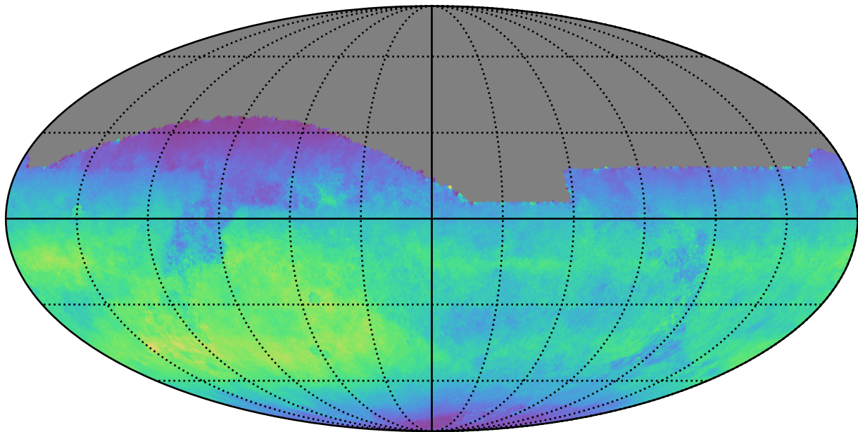
roll_pause_mjdp0_v3.4_10yrs All sky z band: Normalized Teff
