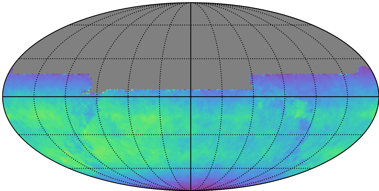
roll_pause_mjdp0_v3.4_10yrs All sky y band: Normalized Teff
