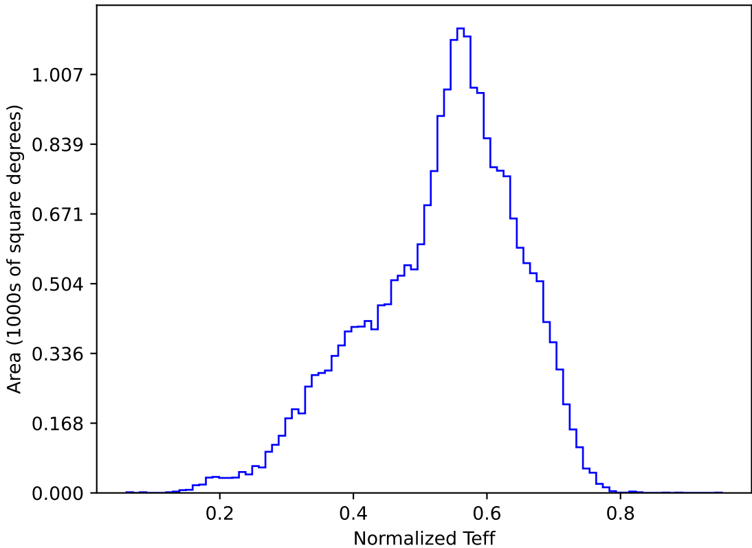
roll_pause_mjdp0_v3.4_10yrs All sky y band: Normalized Teff
