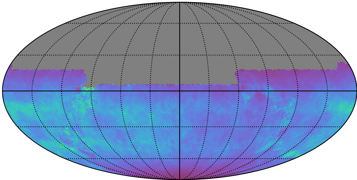
roll_pause_mjdp0_v3.4_10yrs All sky u band: Normalized Teff
