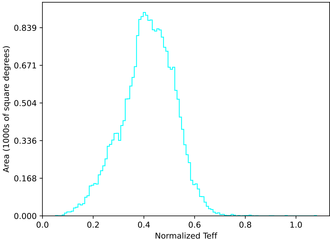
roll_pause_mjdp0_v3.4_10yrs All sky u band: Normalized Teff
