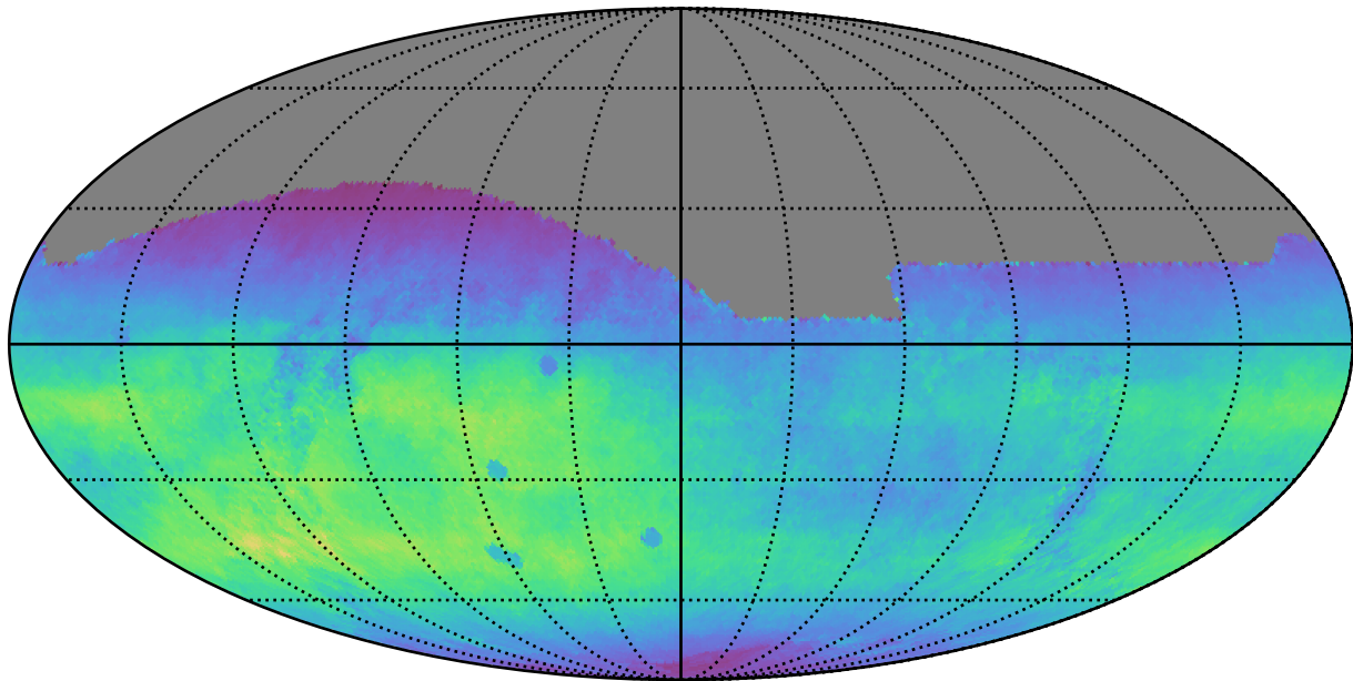
roll_pause_mjdp0_v3.4_10yrs All sky r band: Normalized Teff
