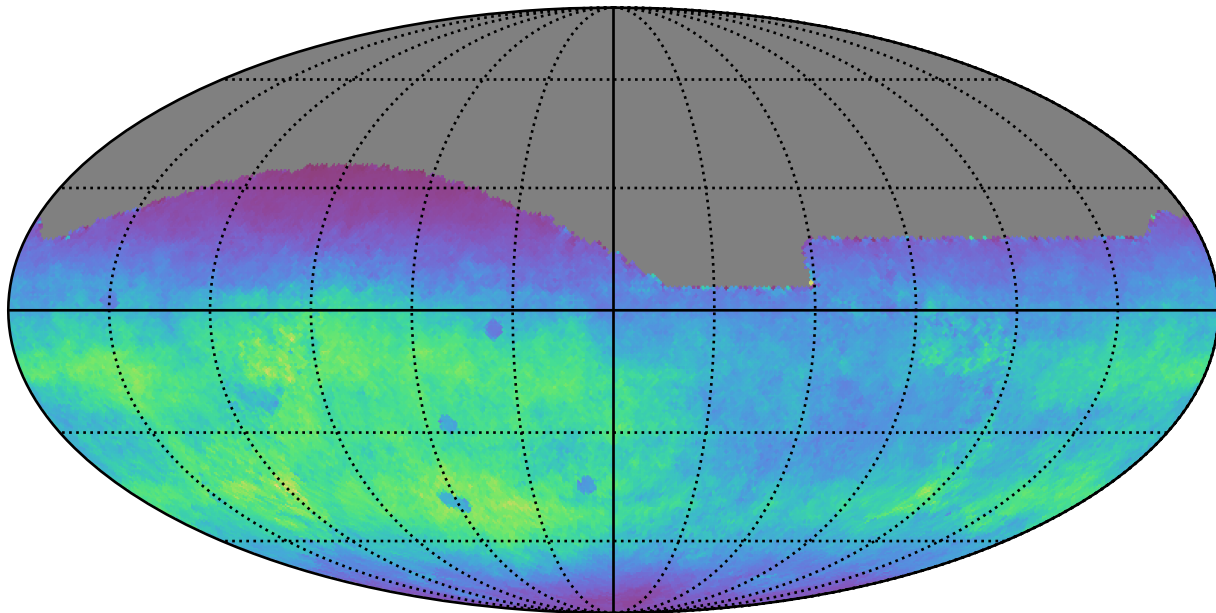
roll_pause_mjdp0_v3.4_10yrs All sky g band: Normalized Teff
