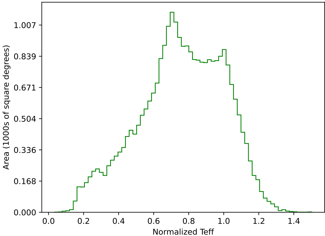
roll_pause_mjdp0_v3.4_10yrs All sky g band: Normalized Teff
