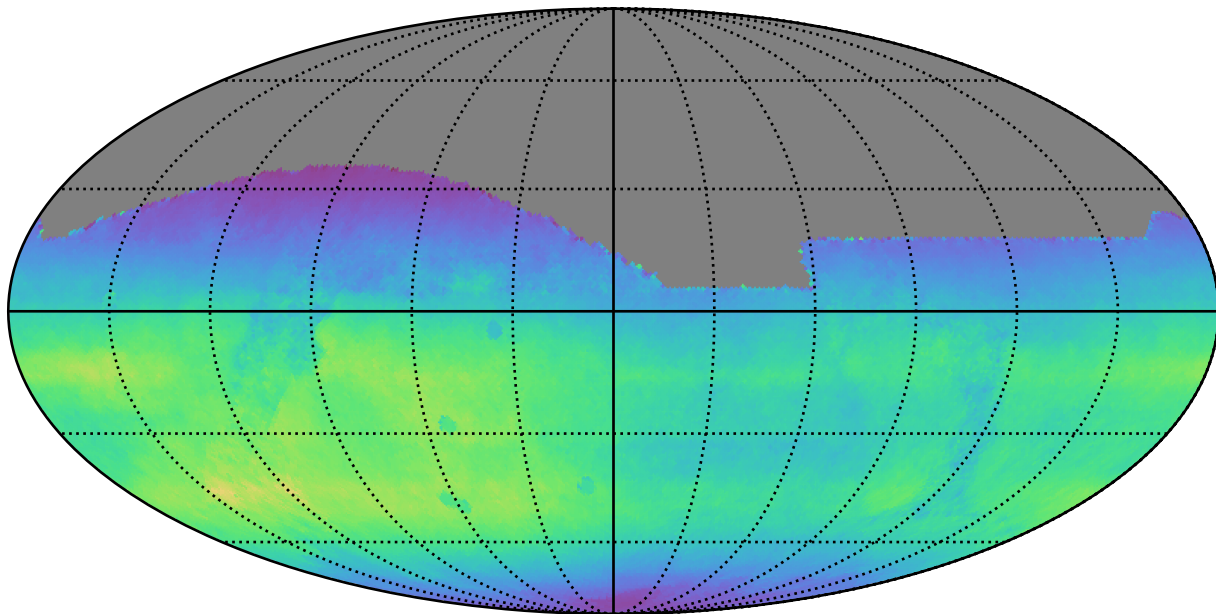
roll_pause_mjdp0_v3.4_10yrs All sky all bands: Normalized Teff
