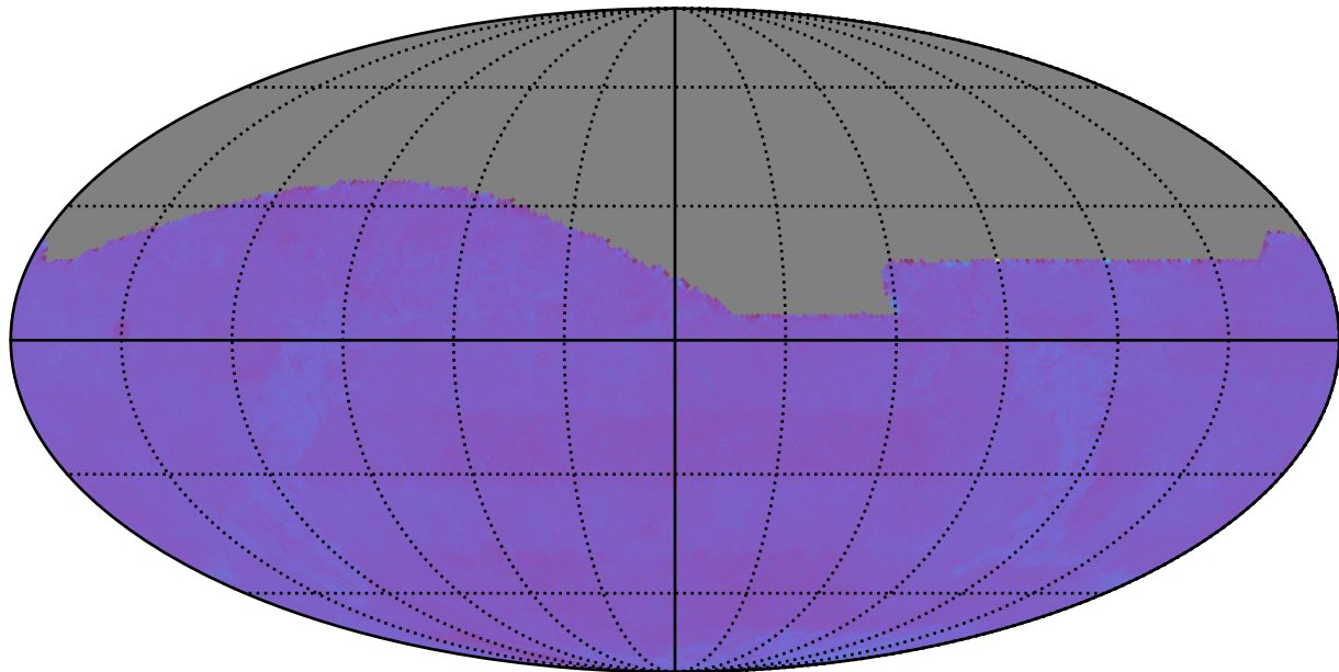
roll_pause_mjdp0_v3.4_10yrs All sky: Normalized Proper Motion Uncert @ 24.0
