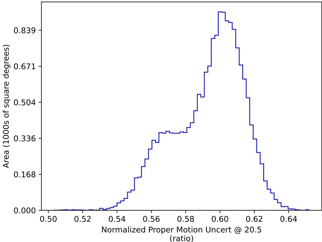
roll_pause_mjdp0_v3.4_10yrs WFD: Normalized Proper Motion Uncert @ 20.5
