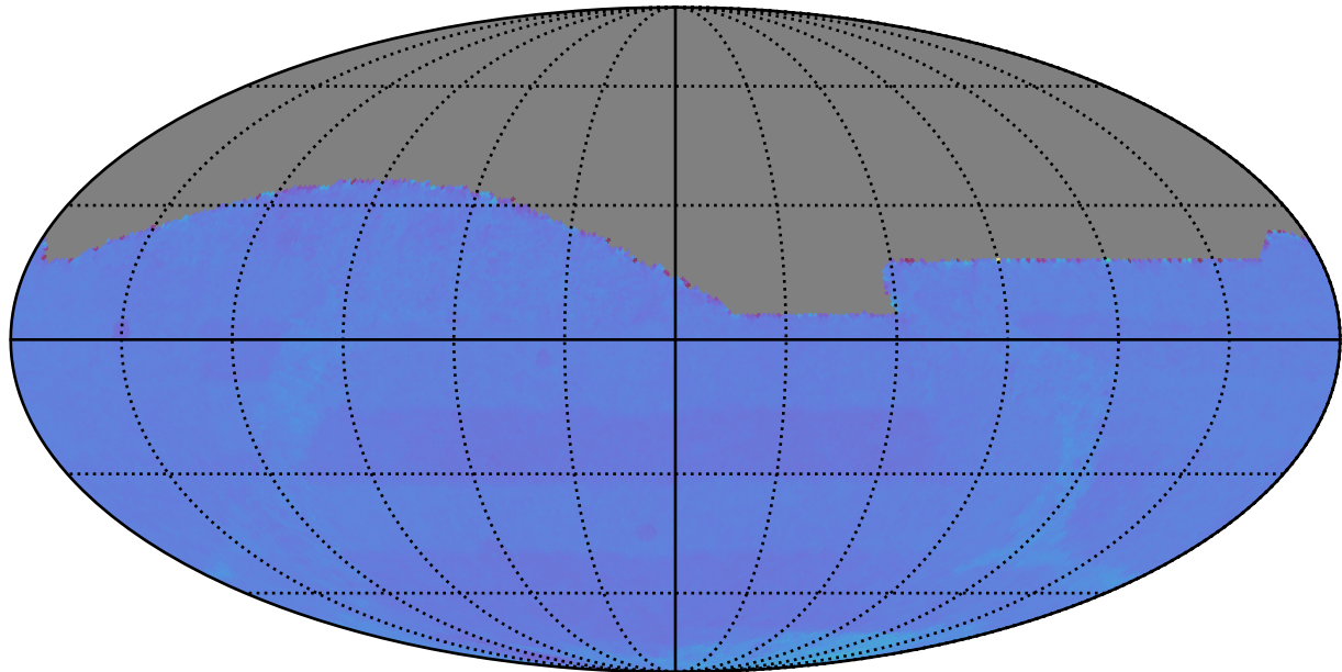
roll_pause_mjdp0_v3.4_10yrs All sky: Normalized Proper Motion Uncert @ 20.5
