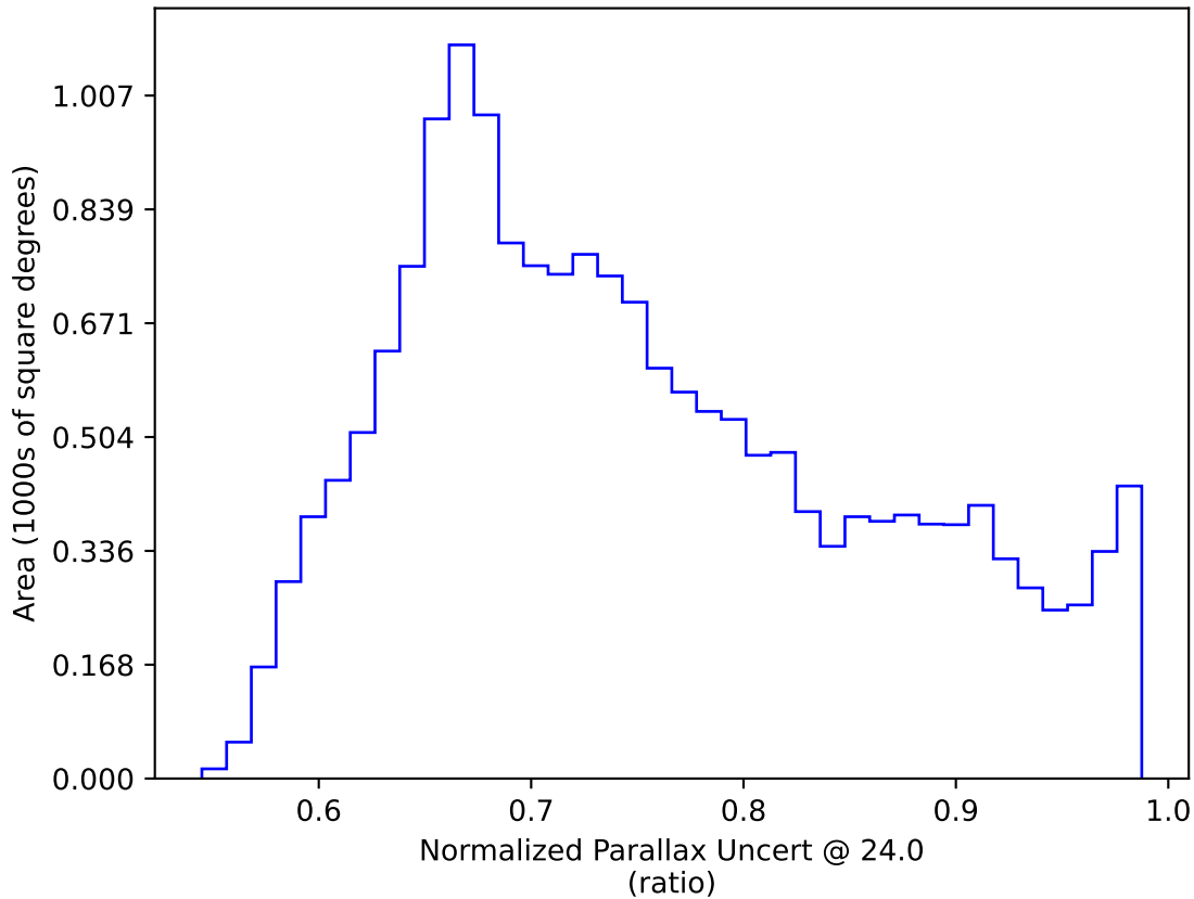
roll_pause_mjdp0_v3.4_10yrs WFD: Normalized Parallax Uncert @ 24.0
