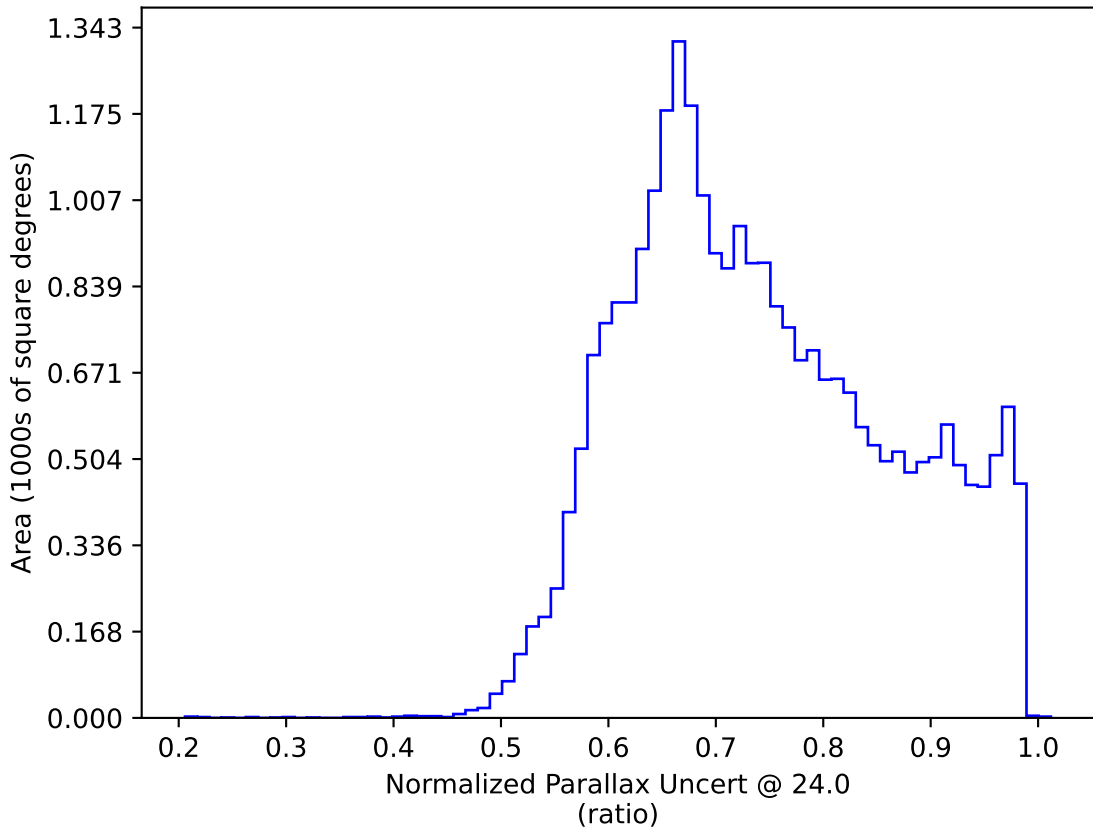
roll_pause_mjdp0_v3.4_10yrs All sky: Normalized Parallax Uncert @ 24.0
