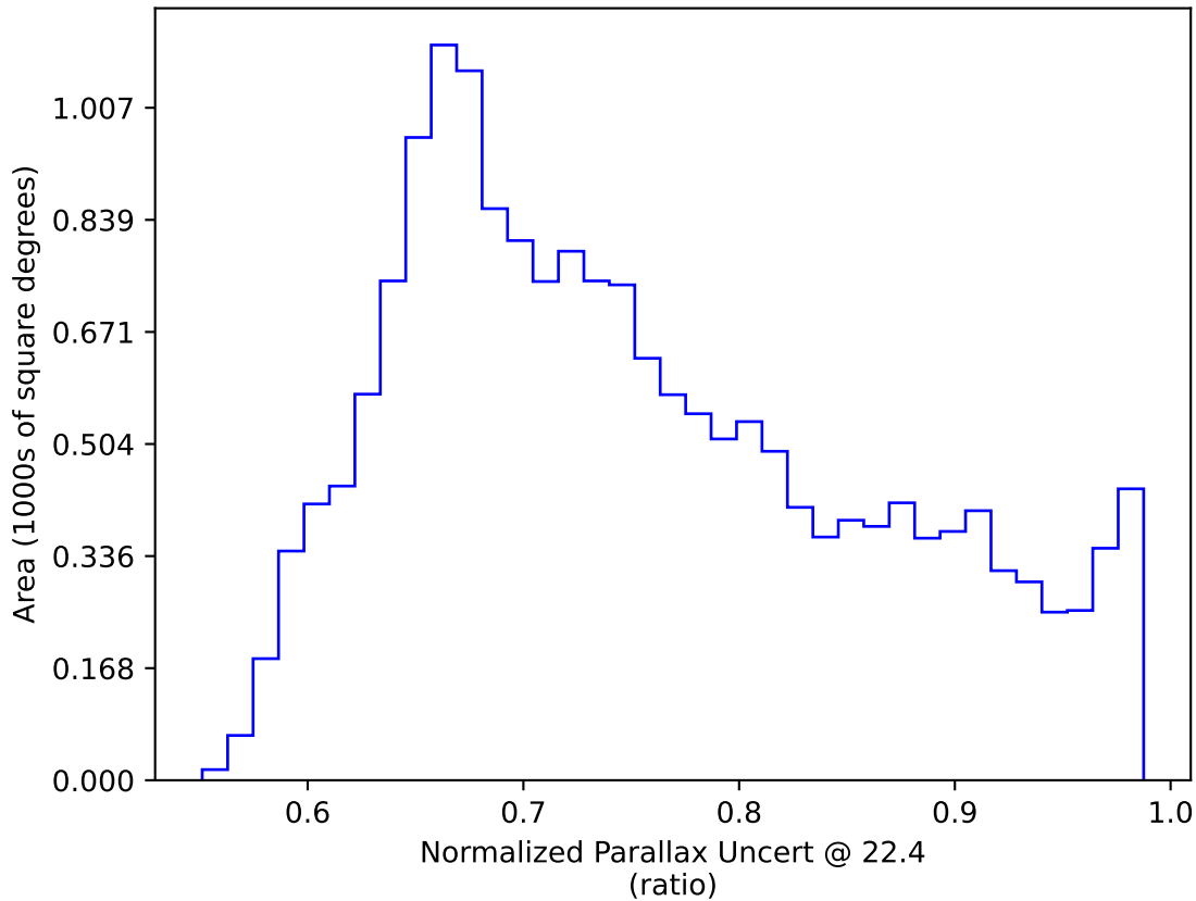
roll_pause_mjdp0_v3.4_10yrs WFD: Normalized Parallax Uncert @ 22.4
