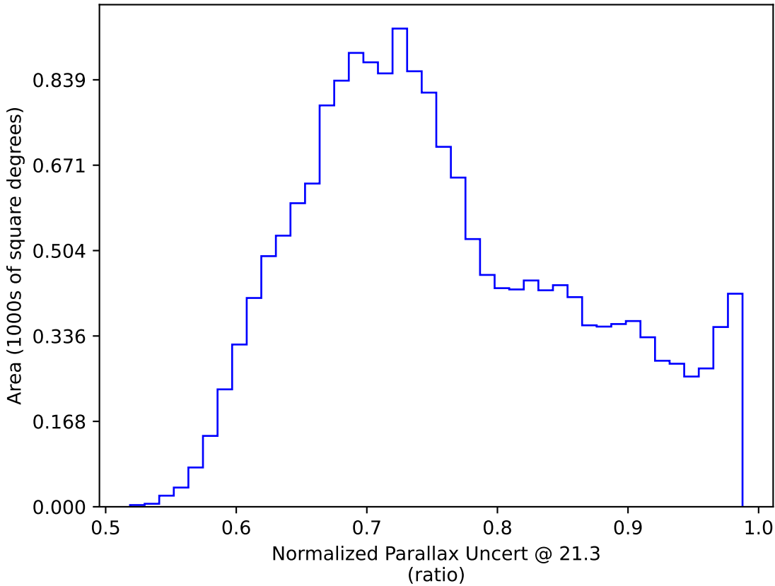
roll_pause_mjdp0_v3.4_10yrs WFD y band only: Normalized Parallax Uncert @ 21.3
