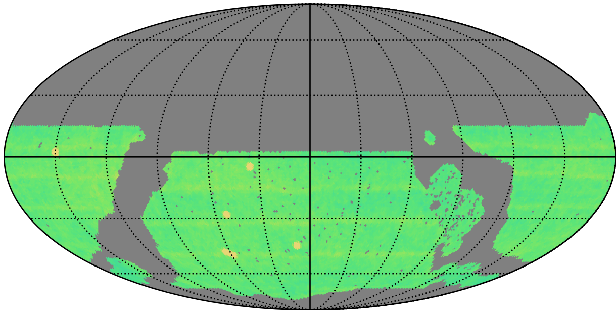
roll_pause_mjdp0_v3.4_10yrs WFD all bands: N Unique Nights
