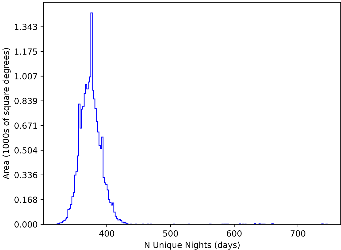
roll_pause_mjdp0_v3.4_10yrs WFD all bands: N Unique Nights
