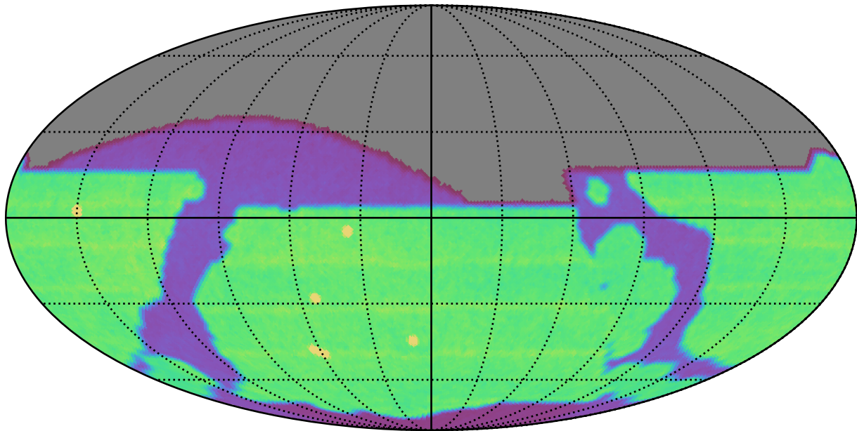
roll_pause_mjdp0_v3.4_10yrs All sky all bands: N Unique Nights
