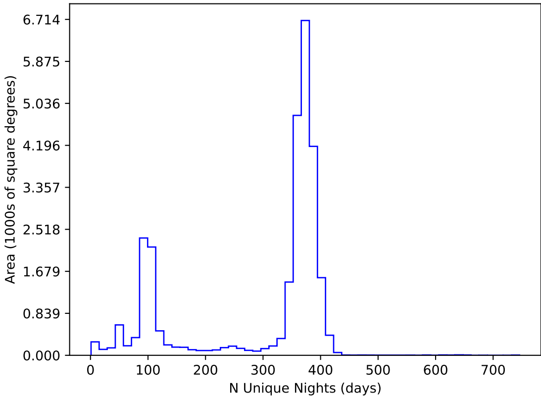
roll_pause_mjdp0_v3.4_10yrs All sky all bands: N Unique Nights
