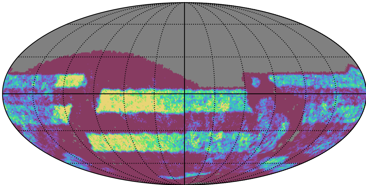
roll_pause_mjdp0_v3.4_10yrs Yr 3-4 z band: NVisits
