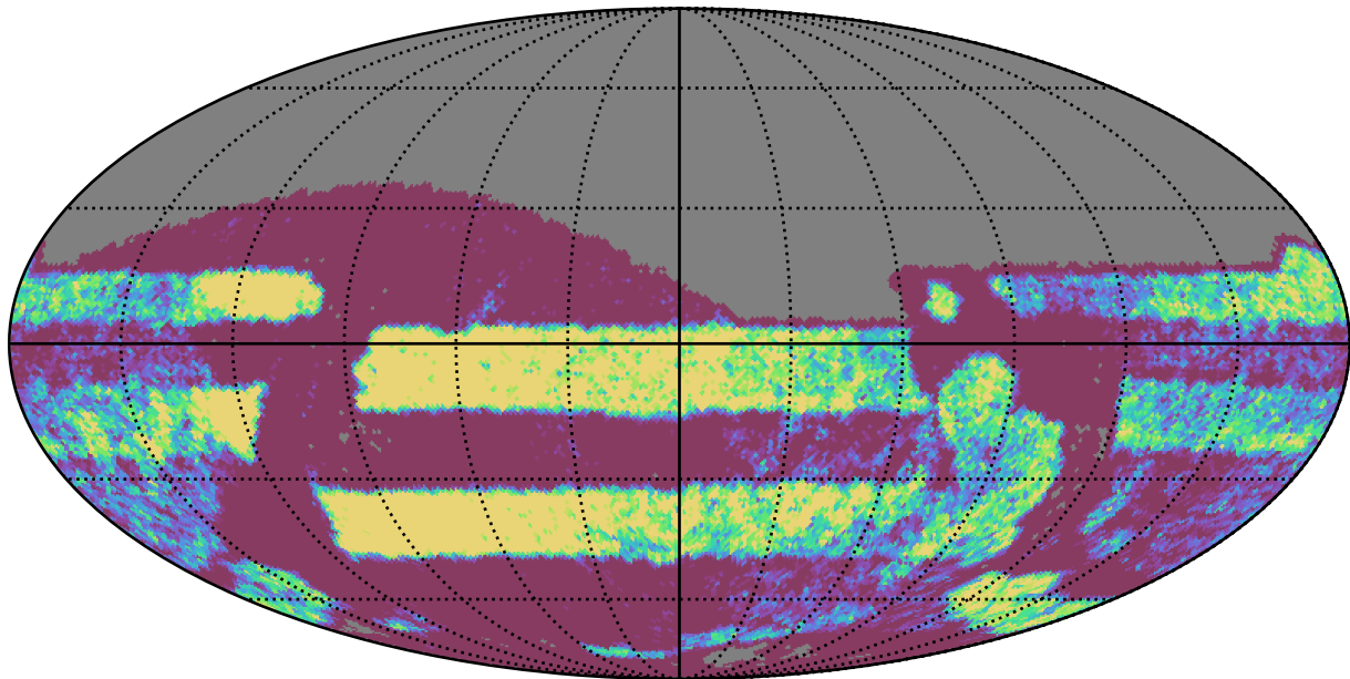
roll_pause_mjdp0_v3.4_10yrs Yr 3-4 r band: NVisits
