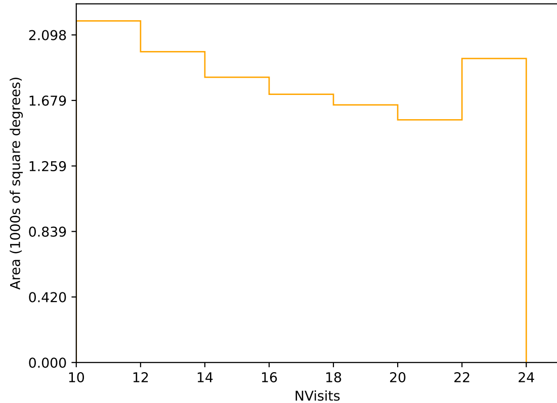
roll_pause_mjdp0_v3.4_10yrs Yr 3-4 r band: NVisits
