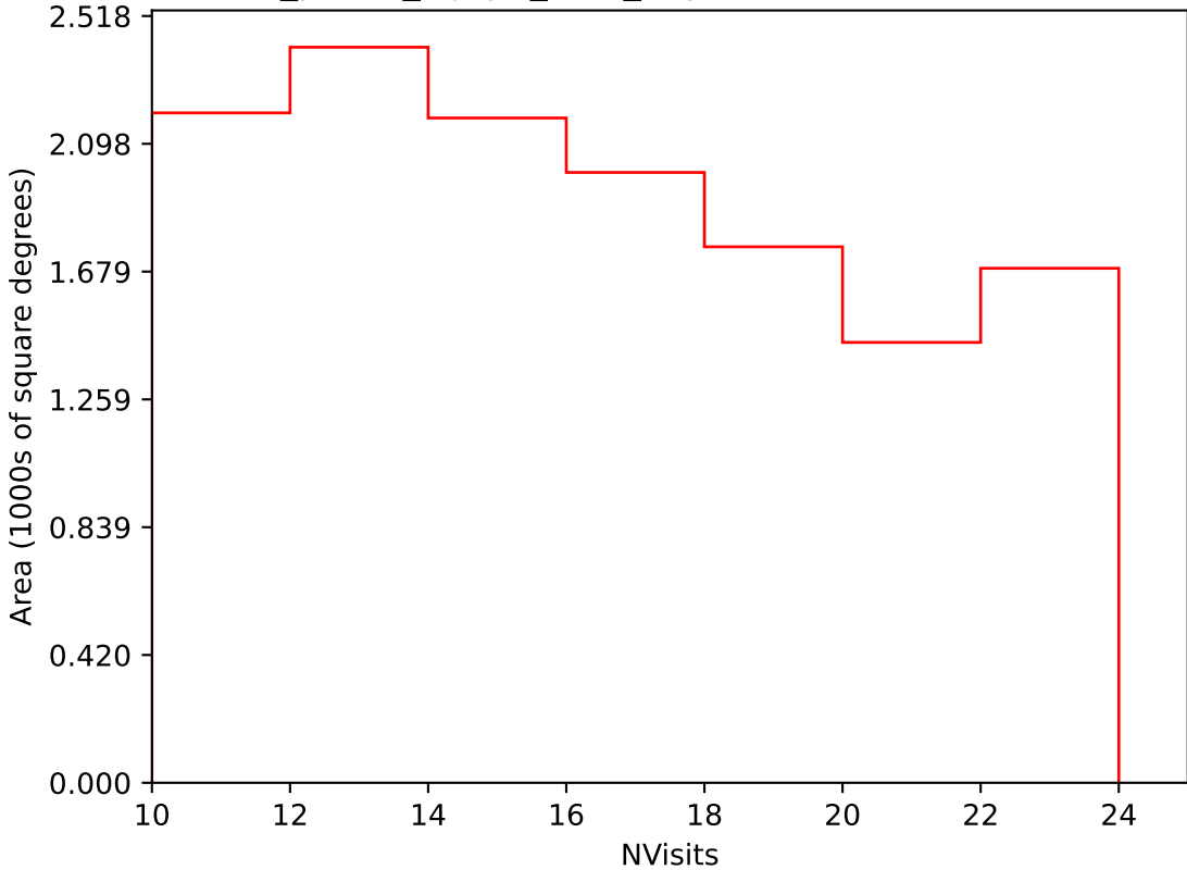
roll_pause_mjdp0_v3.4_10yrs Yr 3-4 i band: NVisits
