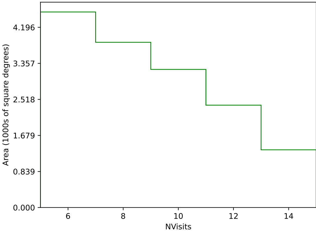
roll_pause_mjdp0_v3.4_10yrs Yr 3-4 g band: NVisits
