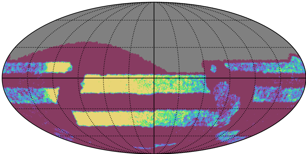
roll_pause_mjdp0_v3.4_10yrs Yr 3-4 all bands: NVisits
